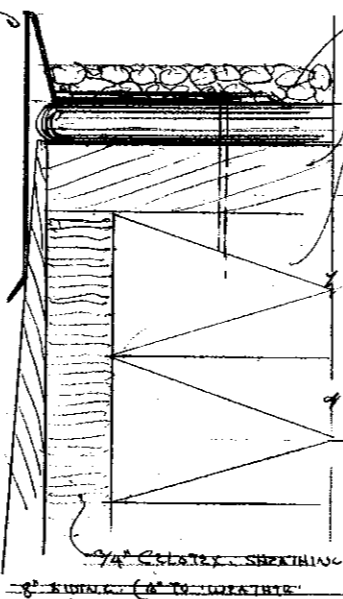
CORNICE DETAIL, F.S.D.
