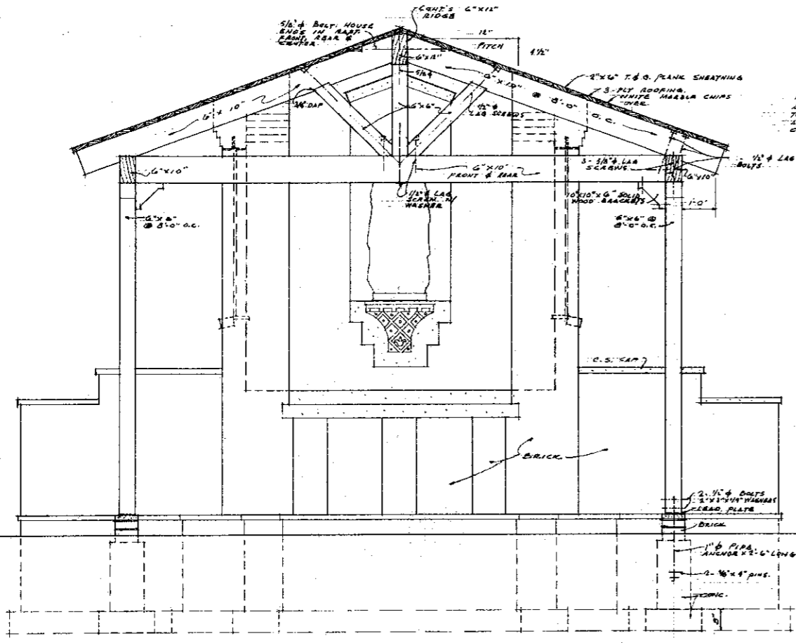
FRONT ELEVATION - SHOWING TRUSSED RAFTER @ FRONT SCALE: 1/2" = 1'-0"
