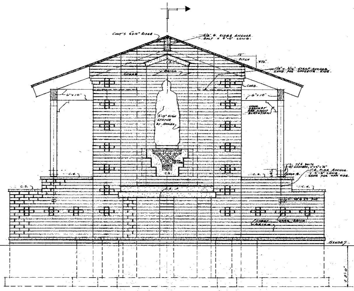
ELEVATION OF ALTAR SCALE: 1/2" = 1'-0"
