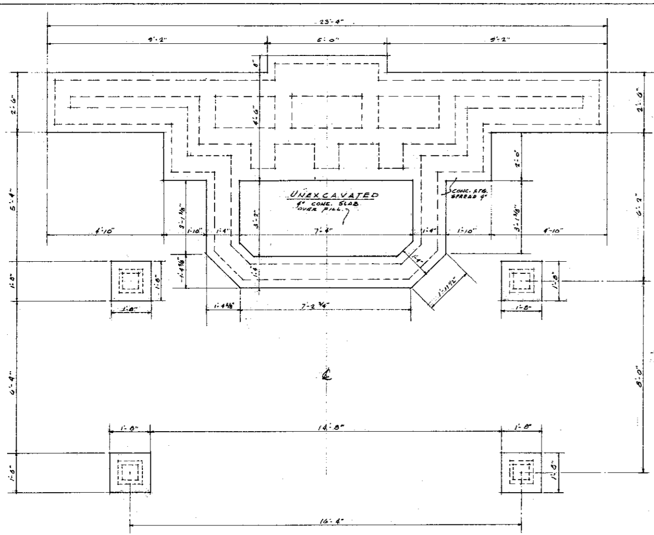
FOOTING PLAN SCALE: 1/2"=1'-0"
