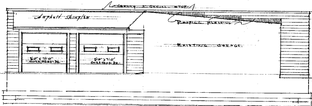
WEST ELEVATION
