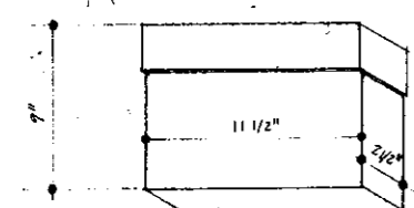
METAL BOX 16" COPPER SOLDER ALL JOINTS
